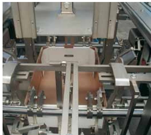
CITRUS + PLATFORM tray hopper Tramoggia per plateau CITRUS + PLATFORM Trichter für Steige CITRUS + PLATFORM Tolva para plateau CITRUS + PLATFORM
